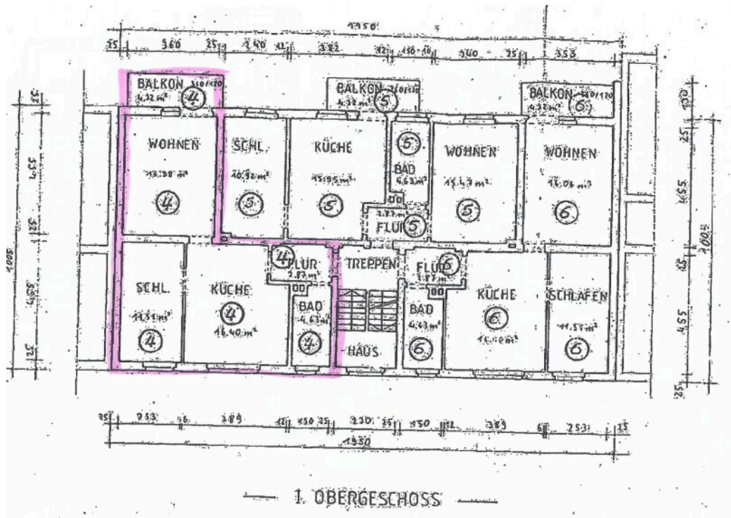
Grundriss - 1.OG links
